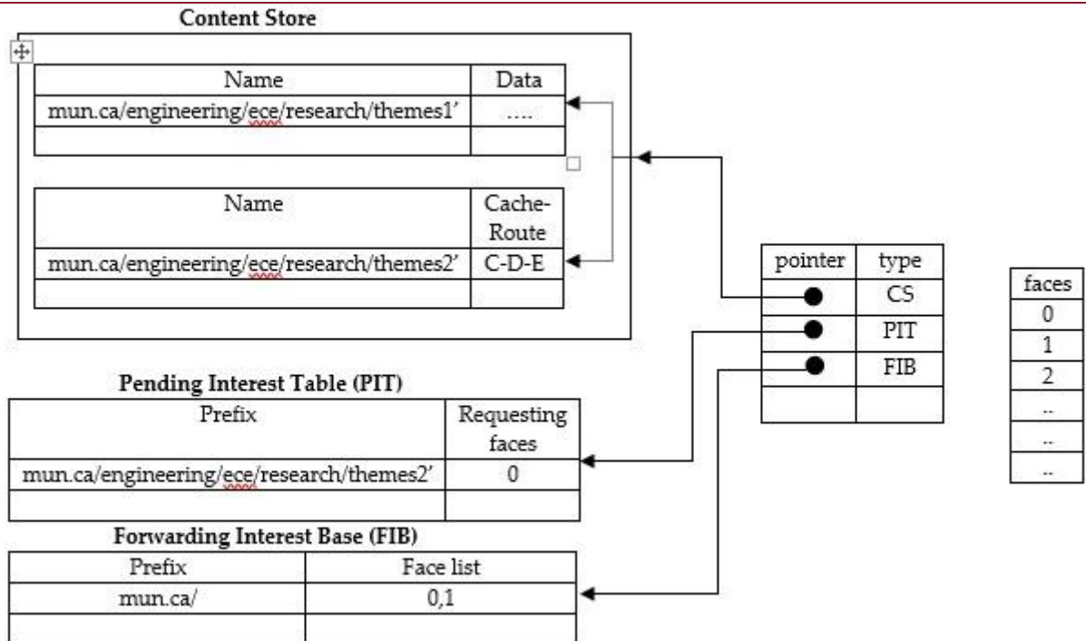
Fig.1 High level view of forwarding engine of Cache-Route strategy
