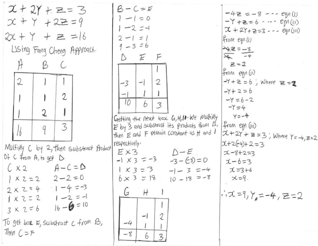
Figure 2. A first-year student’s solution to a system of linear equation using the fang cheng procedure
