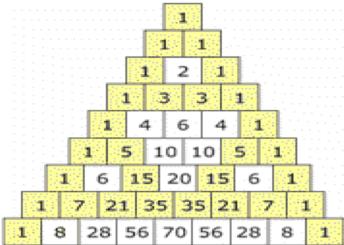
Figure 3. The Meru Prastara
