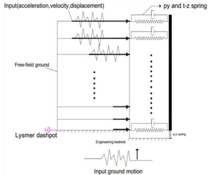
Fig. 6 Method of seismic analysis of pile-soil interaction considering the effect of site response
