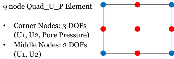
Fig. 5 9-node element with degree of freedom of pore water pressure in corner nodes
