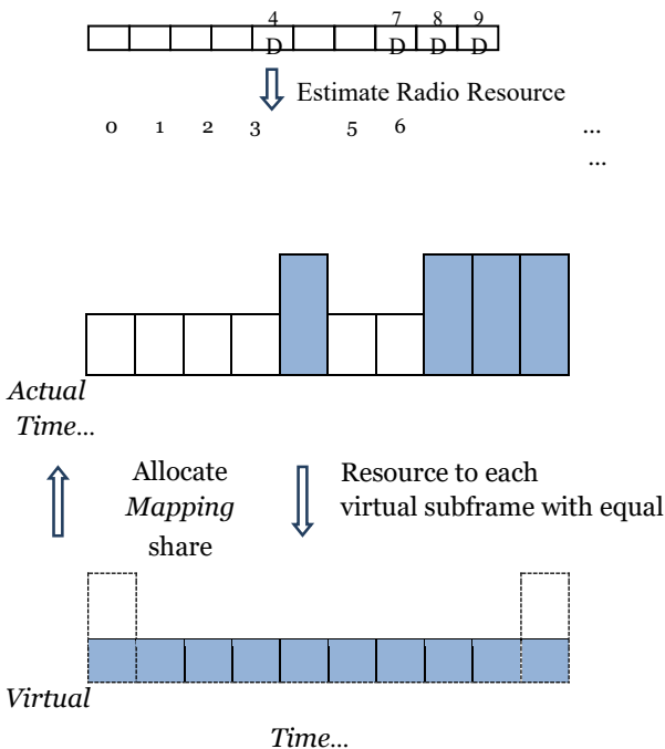
Fig. 3 The idea of Virtual Time
