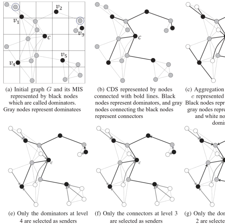
Fig. 4 (a)-(c) Illustration of MIS-based Tree Construction, (d)-(h) Illustration of Scheduling
