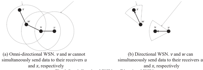
Fig. 1 Omni-directional WSN vs. Directional WSN
