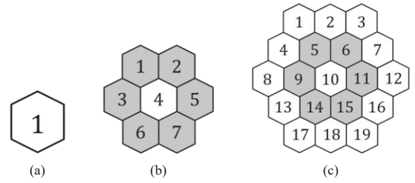
Fig. 3 Coloring by [20]: (a) 1-coloring, (b) 7-coloring, (c) 19-coloring, (d)
