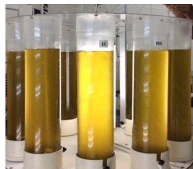
Fig. 2 Photo-bioreactor (patent: Privilege of Innovation, registration
