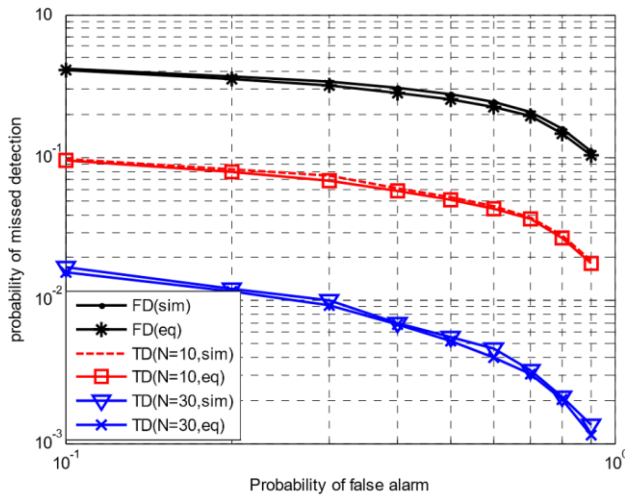
Fig. 3 P_m vs. P_f for approximate analysis
