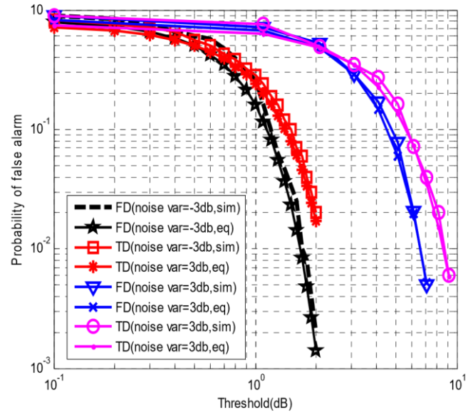
Fig. 7 P_f vs. Threshold for time averaging
