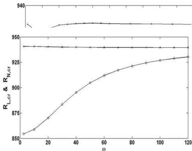
Fig. 1 (a) R_{N,cr} & R_{L,cr} against \omega with a = 0.1, Da = 1, k_r = 0.1 for symmetric modulation
