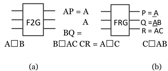
Fig. 1 Block diagrams of (a) F2G, and (b) FRG
