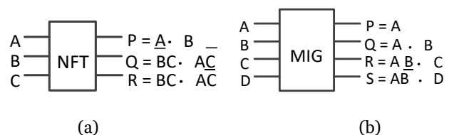
Fig. 2 Block diagrams of (a) NFT, and (b) MIG
