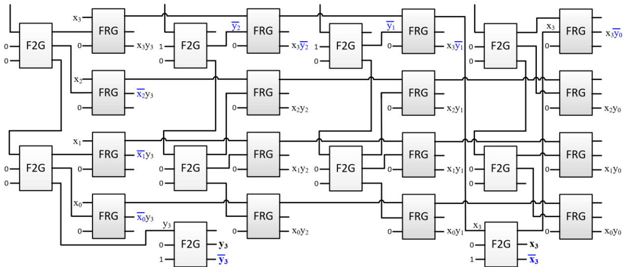
Fig. 7 First proposed 4x4 PPG based on the first Baugh-Wooley method
