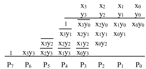
Fig. 6 4x4 signed multiplication based on the second Baugh-Wooley method
