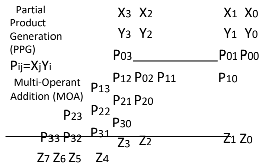
Fig. 4 A 4×4 unsigned multiplier that can be implemented as an array multiplier with two parts
