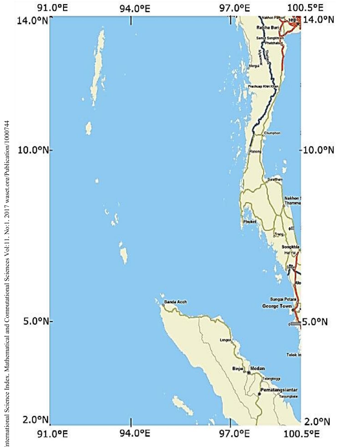
Fig. 3 Model Domain including the coastal geometry and the epicenter of the 2004 earthquake (as [7])
