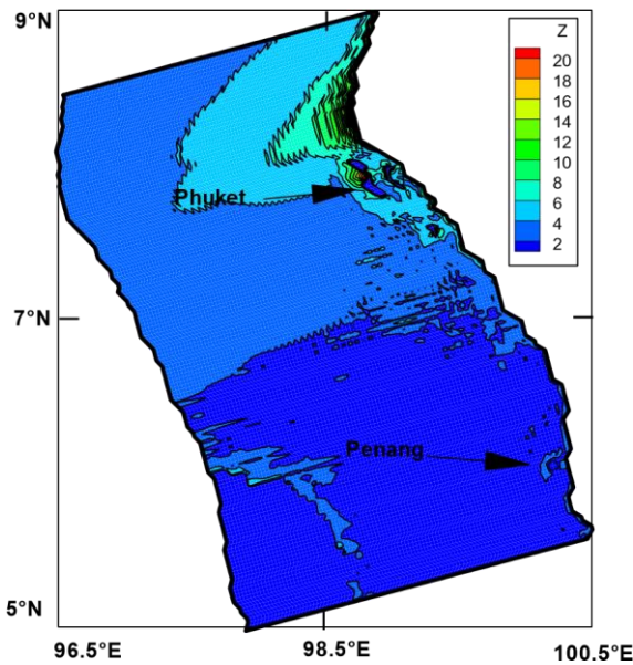
Fig. 6 Contour of maximum water elevation around the west coast of Thailand and Malaysia
