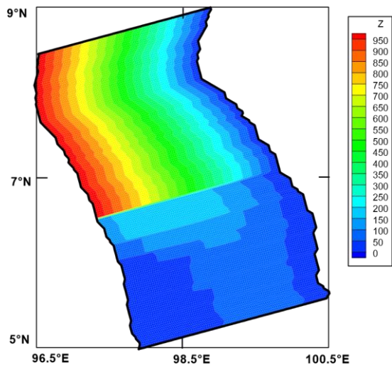
Fig. 4 Bathymetry used during the simulation process
