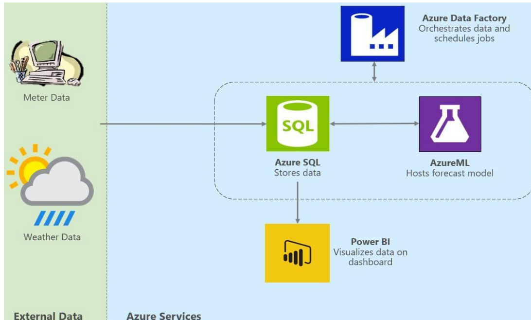
Fig. 8 Solution Architecture
