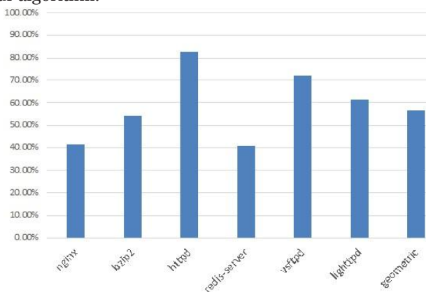
Fig. 5 Result on constraint analysis: the indirect call targets comparing to
