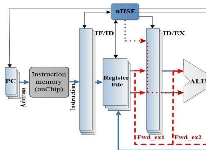
Fig. 1 Replication of resources of the nMPRA architecture and redirecting data in Scheduler Engine, PC: program counter, IF: instruction fetch, ID: instruction d
