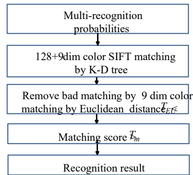
Fig. 7 Flow chart of discarding the unreliable matching
