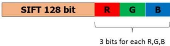
Fig. 6 Moment color-SIFT descriptor with 9-bit RGB format
