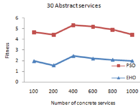
Fig. 5 Fitness evaluation according to number of concrete services
