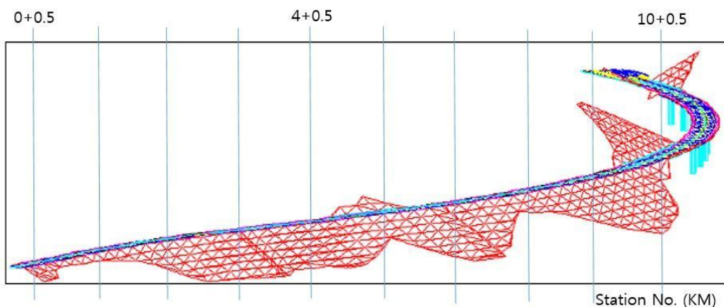
Fig. 4 Earthwork modeling process of natural terrain
