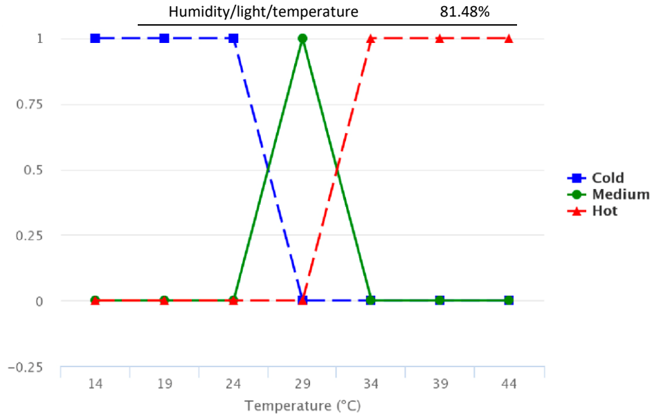
Figure 8. Temperature inference rule.
