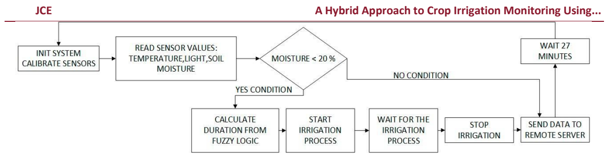
Figure 6. Process workflow: the main loop introduces a time delay in the whole process. Once the sensors are calibrated and measures obtained, the moisture level is checked. If the humidity crosses a given threshold, data is sent to the server. Otherwise, the input values of the sensors are sent to the fuzzy logic algorithm and the irrigation process is triggered.
