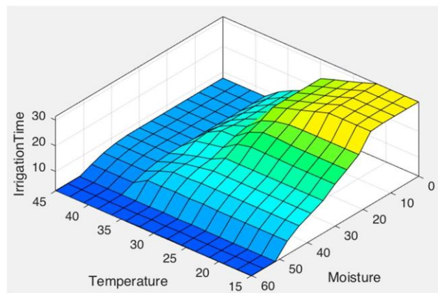
Figure 14. Relation between temperature and moisture.
