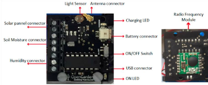
Figure 4. OpenGarden Slave Node functionality board [42].
