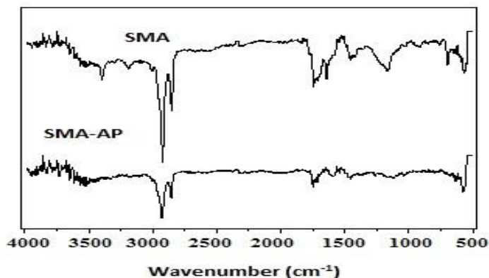
Figure 1: FT-IR spectra of SMA and SMA-AP
