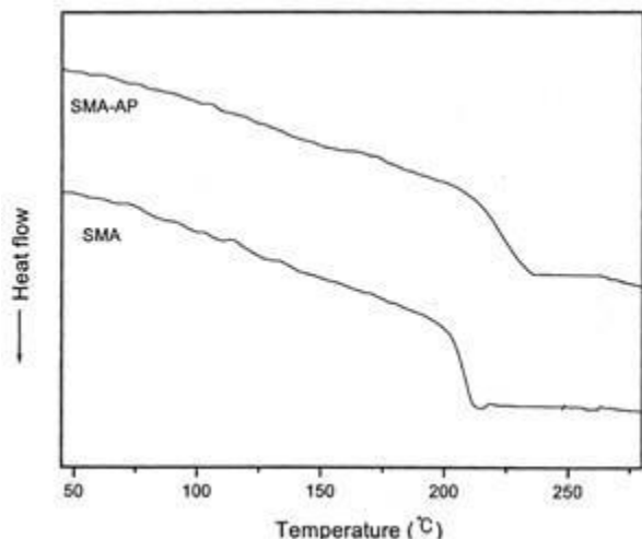
Figure 3: DSC Thermograph for SMA-AP polymer
