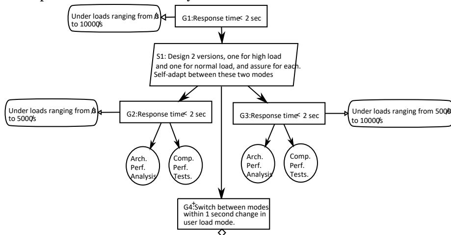
Fig.3. An example Goal Structuring Notation diagram for Znn.
