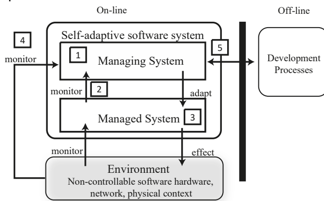
Fig.4. Architectural Reference Model for Self-Adaptive Software Systems.
