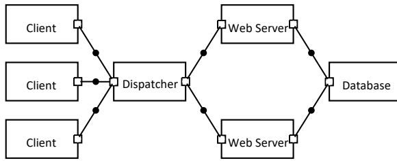
Fig.1. Architecture of the Znn web system.
