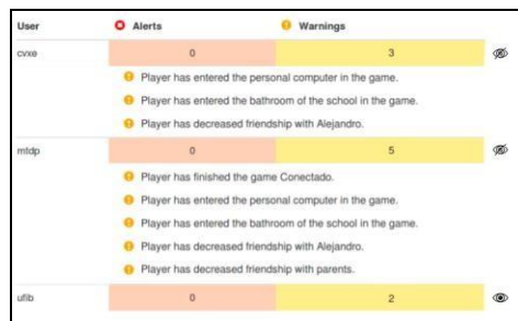
Fig. 4. Previous (top) and updated (bottom) alerts & warnings view. The previous display only counts of alerts and warnings; teachers had to click on student names to view the actual alerts and warnings for those students. The updated version does not require such a context switch.
