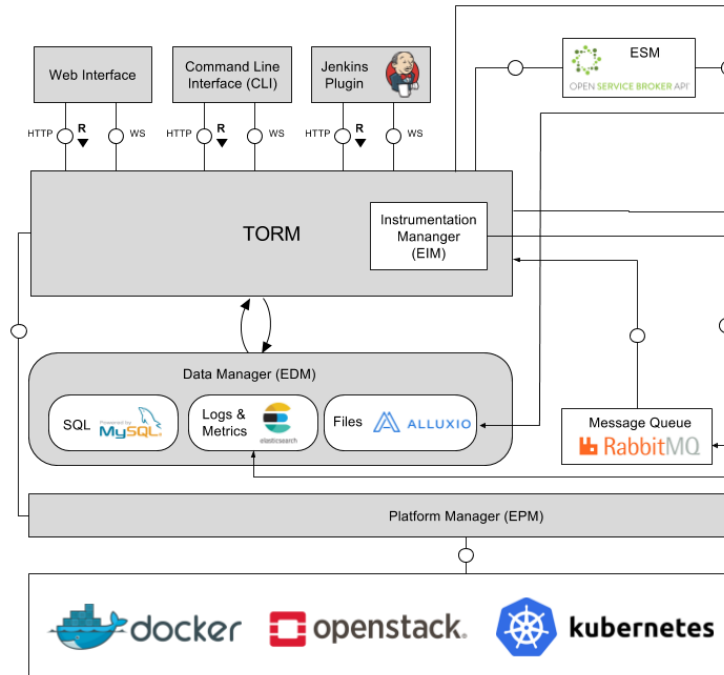
Figure 3: ElasTest architecture
