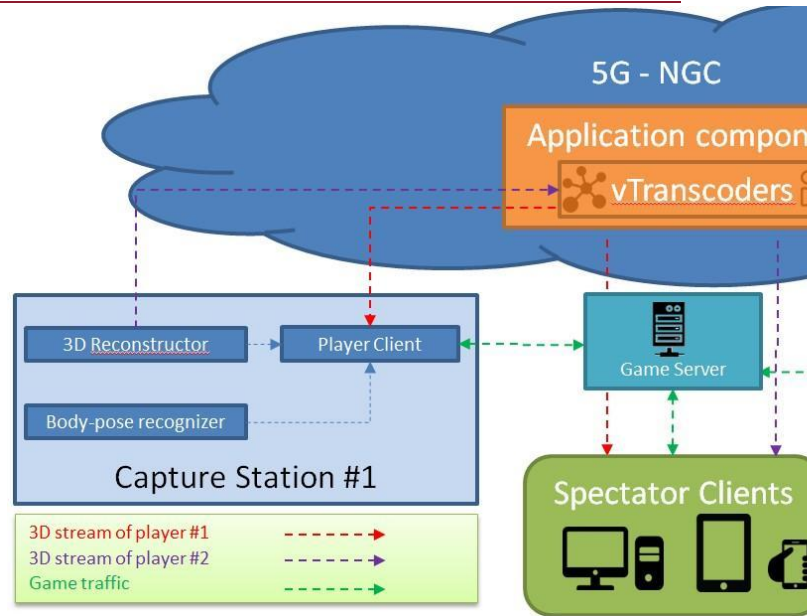
Fig. 2. Logical data-flow between software components
