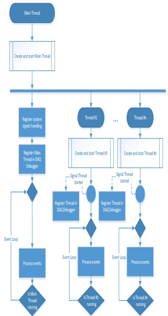
Fig. 4 Flow diagram of the thread registration procedure
