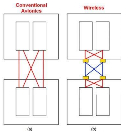
Fig. 2 Redundancy wireless interface design
