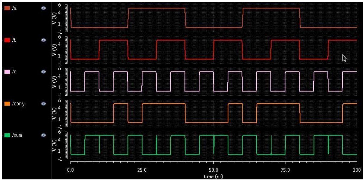
Fig. 4 Waveform of Full adder
