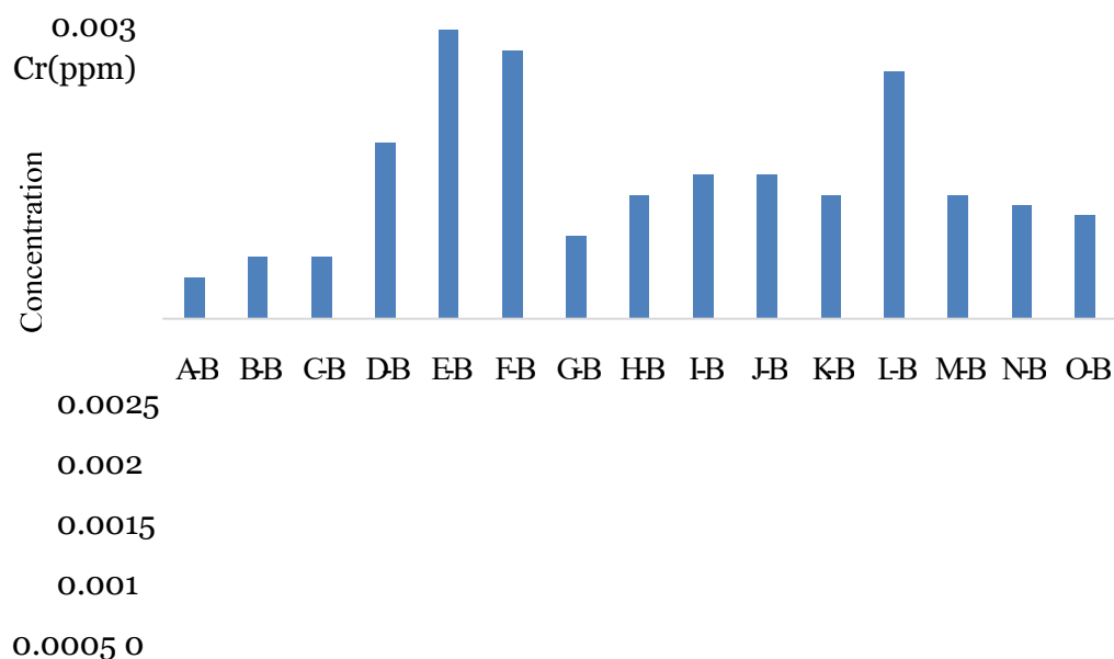
Figure 5: Elemental concentrations (ppm) of Cr in BCM
