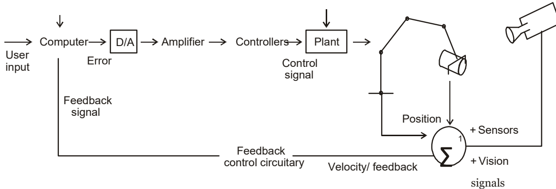
Fig. 3 Block diagram of the robot control system interfaced to the task planner
