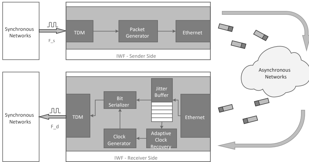
Fig. 1 General structure of a TDMoIP system
