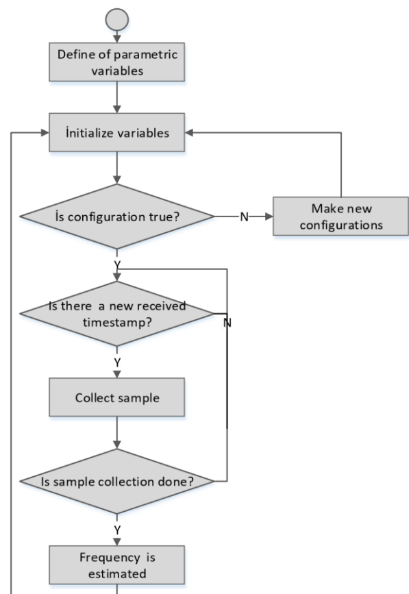
Fig. 3 Algorithm for adaptive clock synchronization RTL
