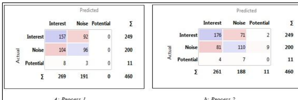
Fig. 5 Comparing performance of the proposed algorithm over current algorithms using confusion matrix Comput. Sci. Appl. J. Comput. Sci. Appl. , vol. 1, no. 3, pp. 39–45, Jan. 2013.
