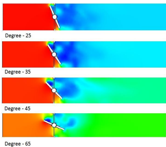
Fig. 6 Pressure distributions of the butterfly valve for various opening angles
