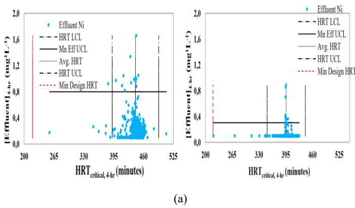
Fig. 11 Critical HRT vs. Effluent Ni Concentration (a) pre-pilot study and (b) post-pilot study
