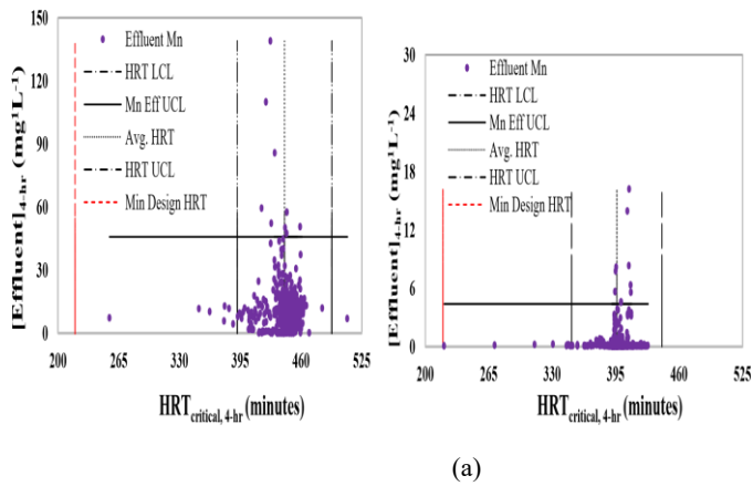
Fig. 12 Critical HRT vs. Effluent Mn Concentration (a) pre-pilot study and (b) post-pilot study
