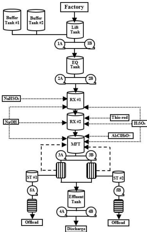
Fig. 2 CCPT Pre-pilot Process Flow Diagram
