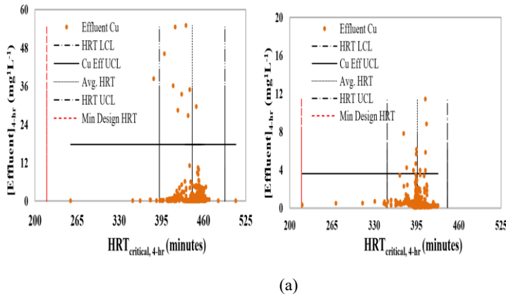
Fig. 10 Critical HRT vs. Effluent Cu Concentration (a) pre-pilot study and (b) post-pilot study
