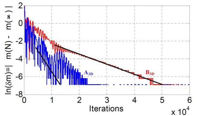
Figure 3: Variation of inlet mass flow rate against iteration number for converged calculations A 3D and B 3D (at 60% blade-speed).
