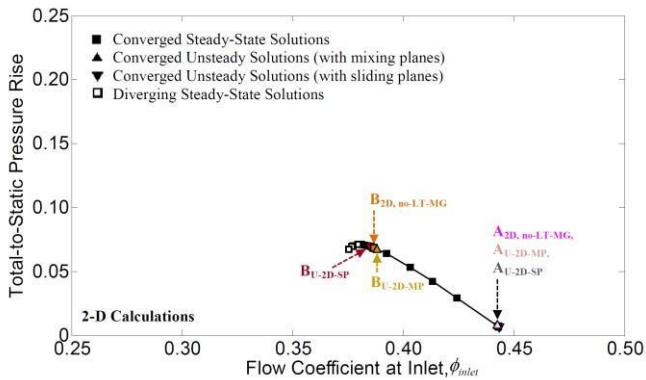
Figure 8: Overall Characteristic for the 2-D midspan section of the IGV+stage1 geometry.
