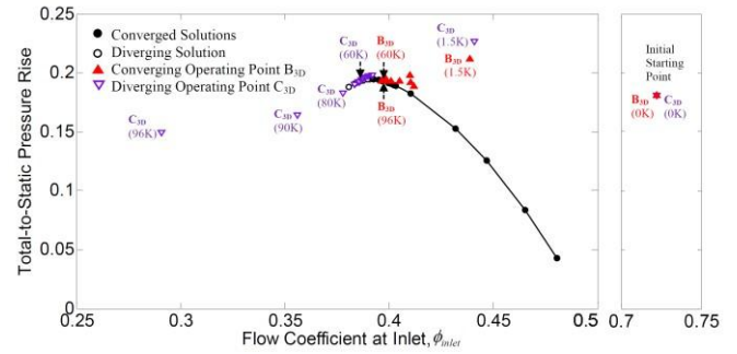
Figure 5: Movement of calculated operating points B_{3D} and C_{3D} with iteration number.
