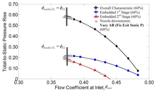
Figure 13: Overall and embedded Characteristics for the IGV+2Stage geometry. Calculations with downstream nozzles are also included.
