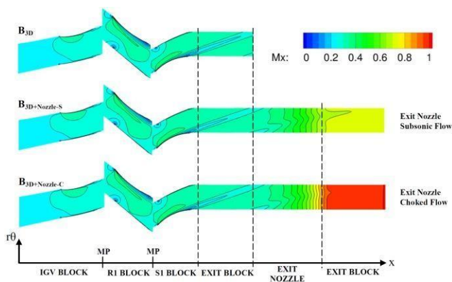
Figure 11: Mid-span blade-to-blade axial Mach number contours for the B_{3D} steady-state operating points shown in Fig. 10.
