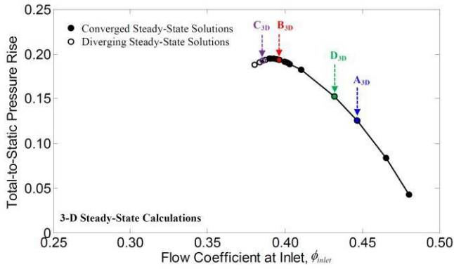
Figure 2: Overall Characteristic for an IGV+1stage generic geometry at 60% blade-speed. Operating points of interest are labelled
