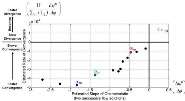
Figure 4: Relationship of convergence rate with the slope of the performance characteristic for the operating points of Fig. 2.
