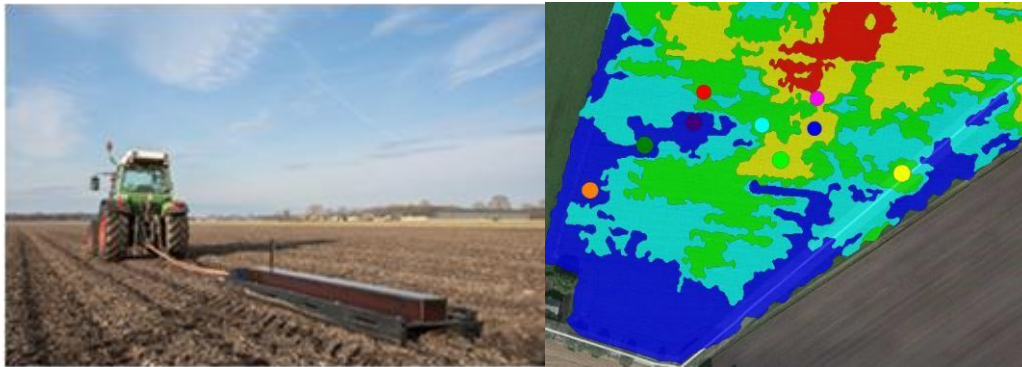
Figure 5. On the left, a tractor scanning the soil with the DualEM sensor. On the right, soil scan result of the pilot field in Netherlands in 2016.
