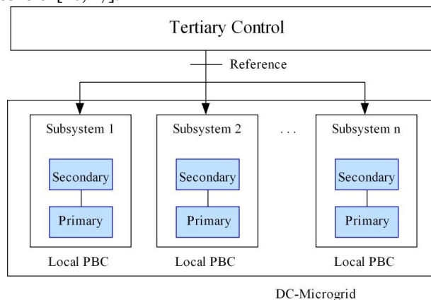
Figure 2 Control structure
