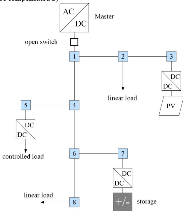
Figure 1 Example of a DC-MG under island operation
