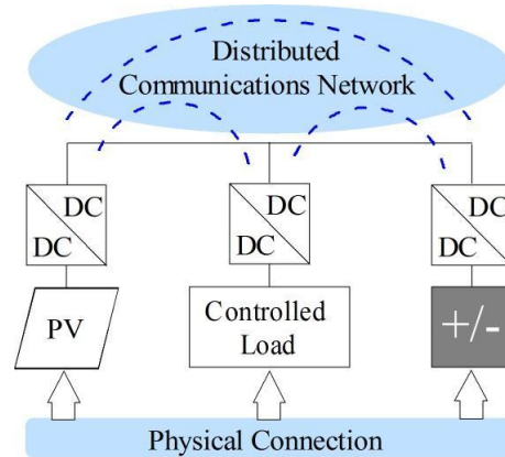
Figure 4 Equivalent DC-MG
