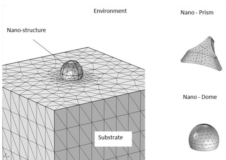
Figure 2. Schematic illustration of the geometry and the mesh elements distribution used for the simulation of Au nano-prism and nano-domes.
