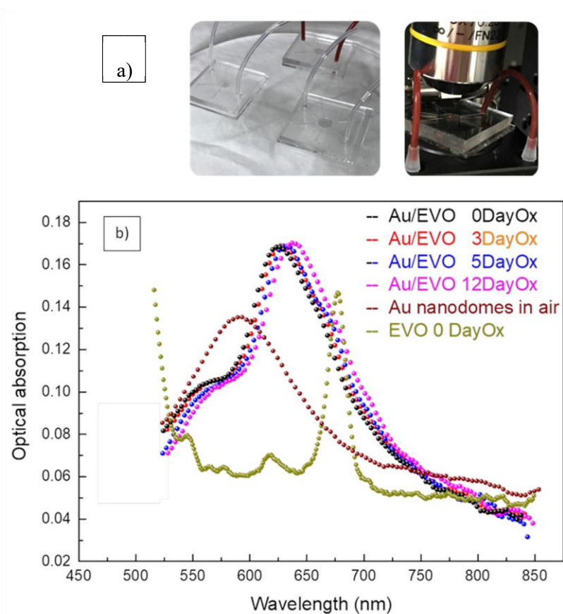
Figure 5. (a) Experimental set-up and microfluidic chips used during the experimental optical measurements (b) Optical absorption measurements in the UV-VIS spectral range performed on EVO oil at different oxidation states. Optical absorption of the nanodomies' array in dry air and of the EVO oil are reported.
