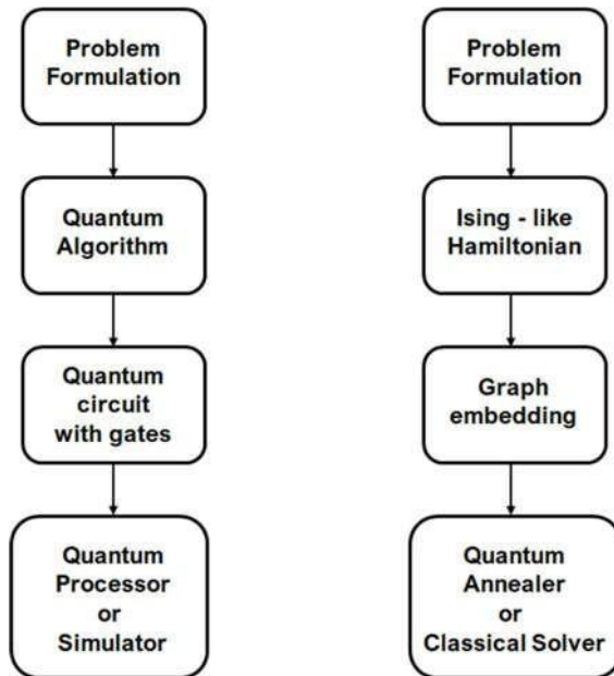
Figure 6. Quantum algorithms workflows: on a gate-model computer (left), on a quantum annealer (right).
