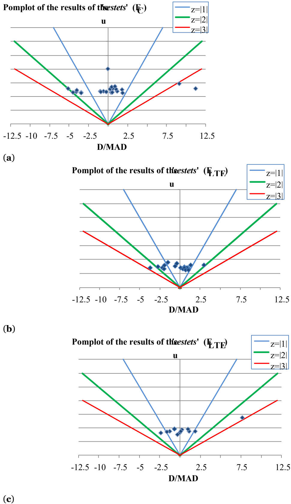
Figure 7. PompPlots of the results of the 'sestets' in the three modalities: (a) E_{CP} . (b) E_{LTE\_RS} . (c) ELTE\_SZ .
