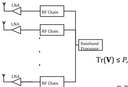
Fig. 2. Fully-digital FS beamforming. In contrast to an all-analog scheme, this architecture spatially processes the data in a baseband processor which offers a large flexibility in terms of operations.
