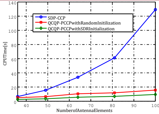
Fig. 5. Average CPU time versus number of antennas for phase-only transmit optimization problem.
