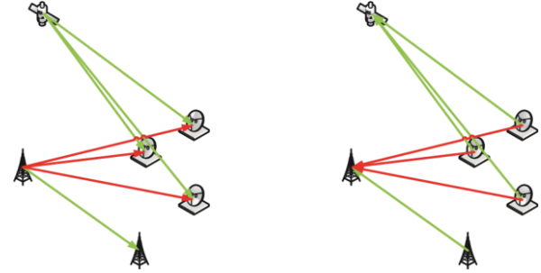
Fig. 1. Schematic of the considered scenarios where the red lines represent the interference signals and the green ones the legitimate transmissions. On the left it is depicted the 18 GHz band case where the FS interfere with the VSATs. Figure on the right describes the 28 GHz shared band case where the VSATs interfere the FS links.
