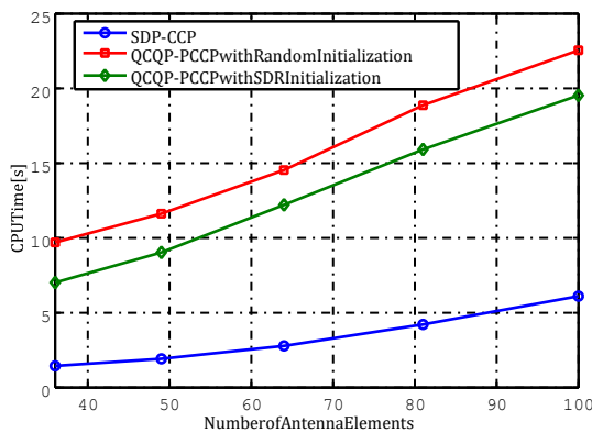
Fig. 8. Average CPU time versus number of antennas for phase-only receive optimization problem.
