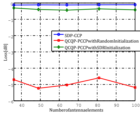
Fig. 4. Performance Loss for phase-only transmit beamforming optimization problem.
