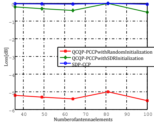
Fig. 7. Performance Loss for phase-only receive beamforming optimization problem.
