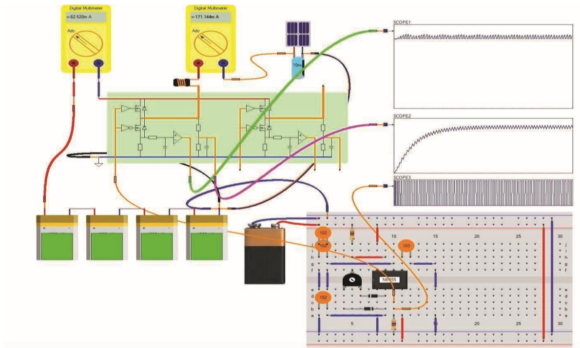
Fig. 7. Combining the U4L with analog circuits constructed on a breadboard.
