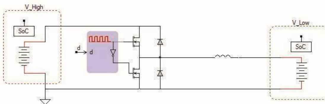
Fig. 3. Battery charging and discharging topology.
