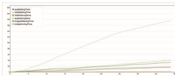
Fig. 2. Resource management
