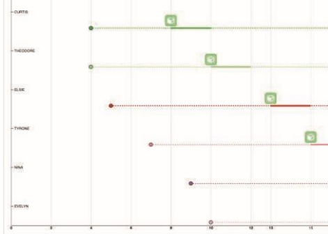
Fig. 2. Resource management
