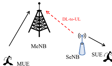
Figure 2. Target scenario composed of a MeNB receiving in UL and a SeNB transmitting in DL. Interference suppression will be implemented at the MeNB to decode and subtract the signal received from the SeNB.
