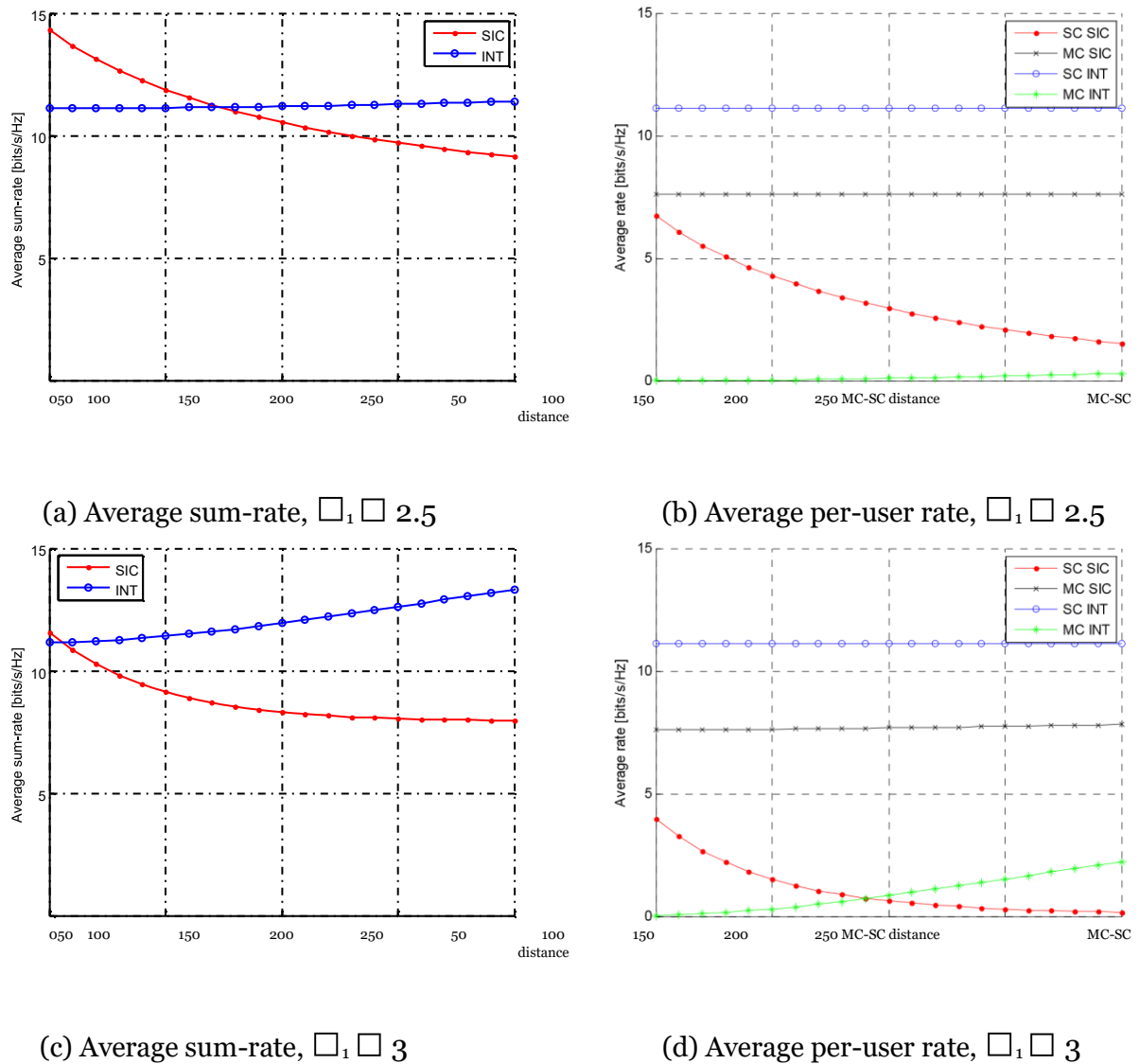
Figure 4. Average sum-rate and average per-user rate (in bits/s/Hz) vs. MeNB-SeNB distance ( d_{SeNB-MeNB} ) under interference conditions ('INT') and the proposed SIC strategy ('SIC') for P_{SeNB} = 24 dBm and different SeNB-MeNB path loss exponents ( \alpha_1 ).
