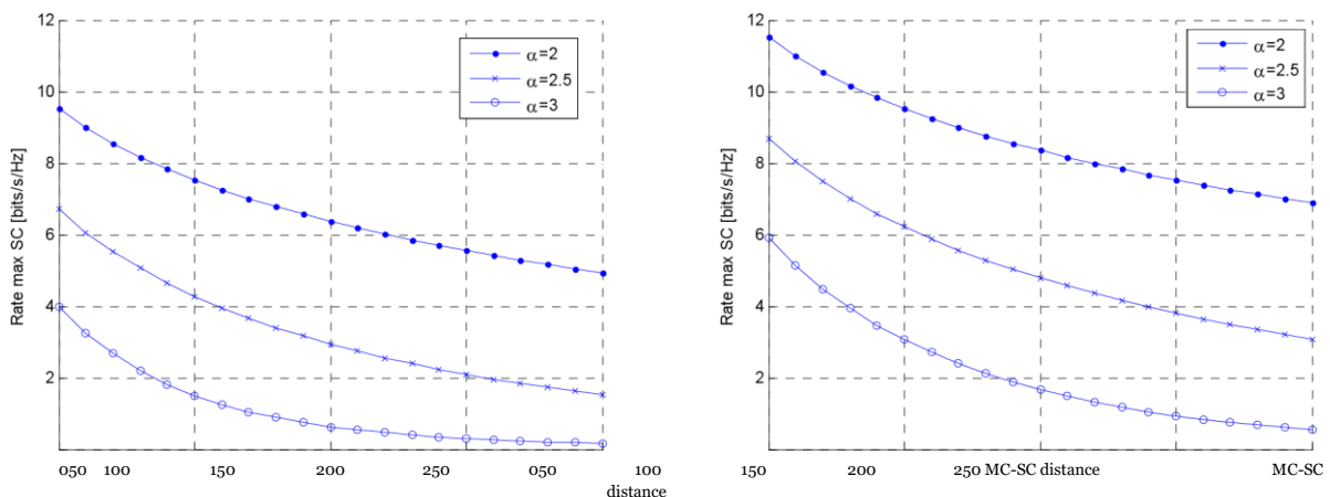
(a) P_{SeNB} = 24 dBm
