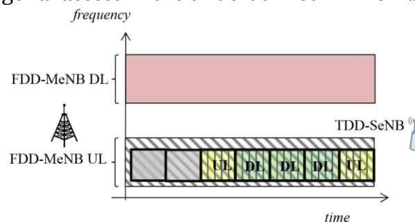
Figure 1. Non-orthogonal access between MeNB and SeNB in the licensed bandwidth for FDD-UL.
