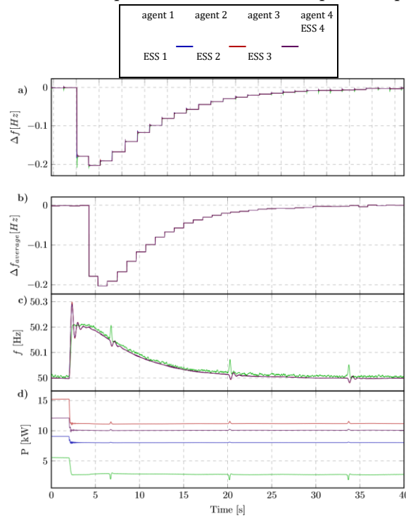
Figure 14. Scenario 5. (a) The state values of agents; (b) Consensus values sent to controllers from agents; (c) Frequency values measured at output of ESSs; and (d) Active power output of ESSs.
