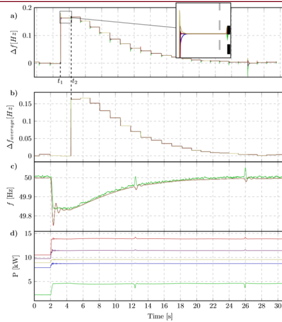
Figure 9. Scenario 1. (a) The state values of agents; (b) Consensus values sent to controllers from agents; (c) Frequency values measured at output of ESSs; and (d) Active power output of ESSs.
