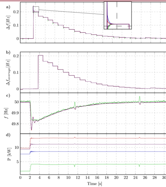
Figure 12. Scenario 3. (a) The state values of agents; (b) Consensus values sent to controllers from agents; (c) Frequency values measured at output of ESSs; and (d) Active power output of ESSs.
