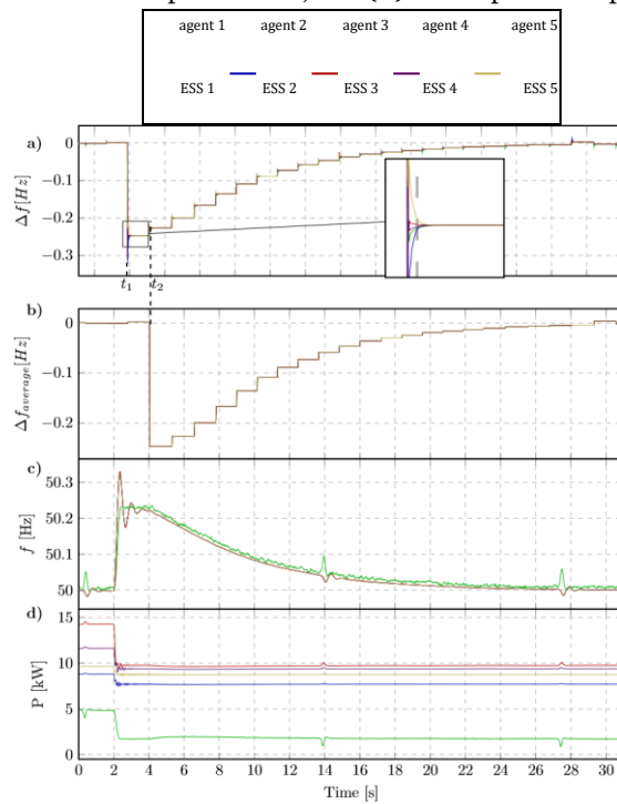
Figure 10. Scenario 2. (a) The state values of agents; (b) Consensus values sent to controllers from agents; (c) Frequency values measured at output of ESSs; and (d) Active power output of ESSs.
