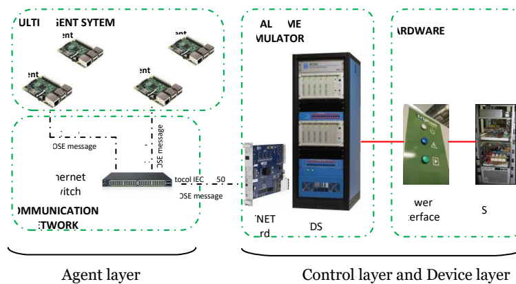
Figure 6. The designed laboratory platform.
