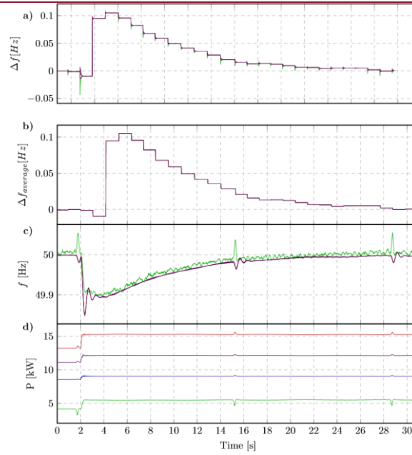
Figure 13. Scenario 4. (a) The state values of agents; (b) Consensus values sent to controllers from agents; (c) Frequency values measured at output of ESSs; and (d) Active power output of ESSs.
