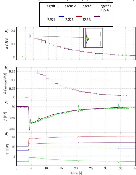
Figure 18. Scenario 7. (a) The state values of agents; (b) Consensus values sent to controllers from agents; (c) Frequency values measured at output of ESSs; and (d) Active power output of ESSs.
