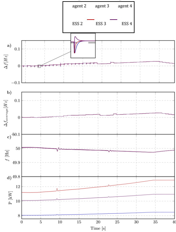
Figure 16. Scenario 6. (a) The state values of agents; (b) Consensus values sent to controllers from agents; (c) Frequency values measured at output of ESSs; and (d) Active power output of ESSs.
