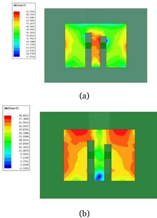
Fig. 6. Simulated surface current distribution of the best design (a) at 25 GHz, and (b) at 37 GHz.
