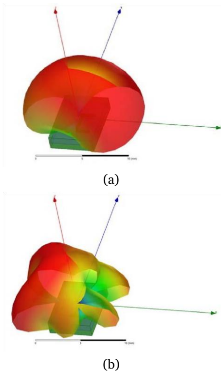
Fig. 5. 3D Radiation pattern of the best design (a) at 25 GHz, and (b) at 37 GHz.
