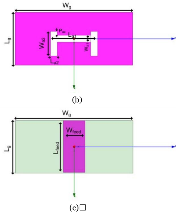
Fig. 2. Geometry of an aperture coupled E-shaped patch antenna a) Patch plane, b) ground plane with aperture and c) feed line plane.
