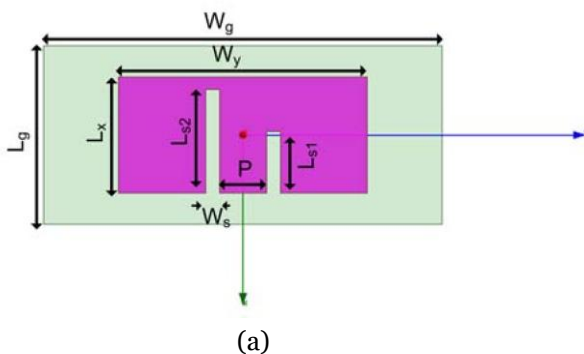
Fig. 1. Geometry of an aperture coupled E-shaped patch antenna
