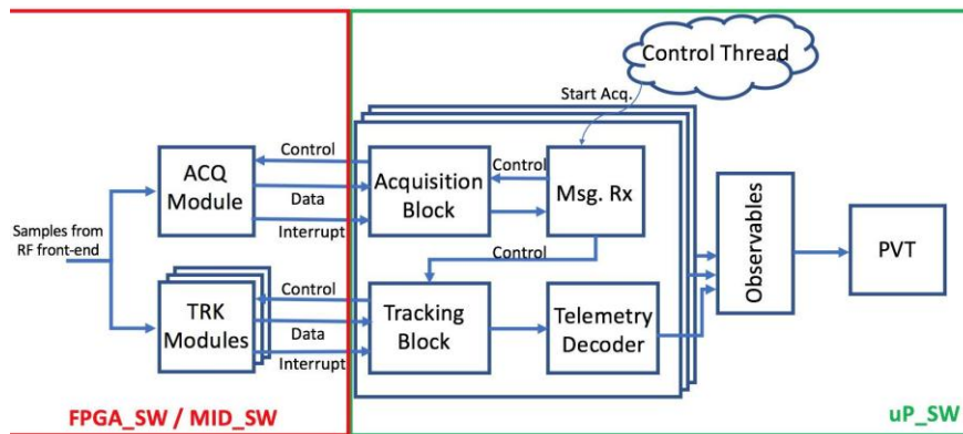
Fig. 3. Architecture of the GNSS-SDR software.
