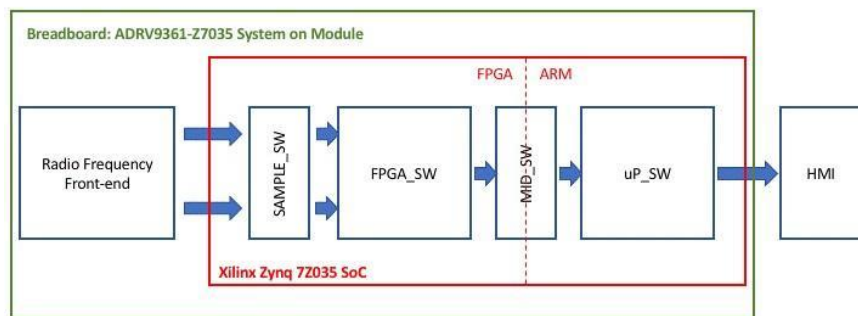
Fig. 1. All-Programmable System-On-Chip.
