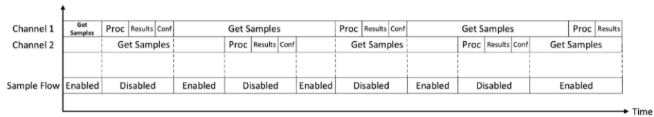
Fig. 11. Timing diagram of two tracking HW accelerators working simultaneously.
