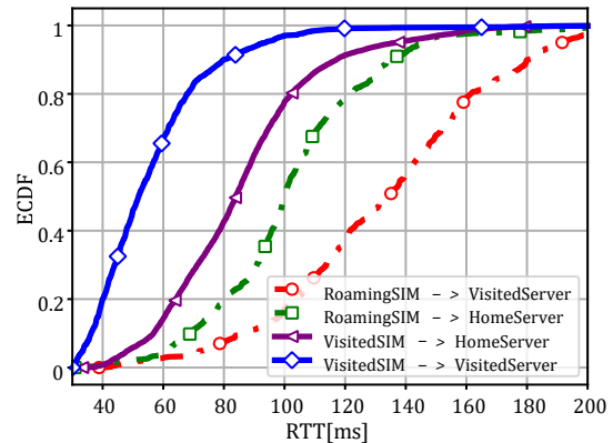
Figure 4: ECDF of the RTT from mobile nodes to target servers.
