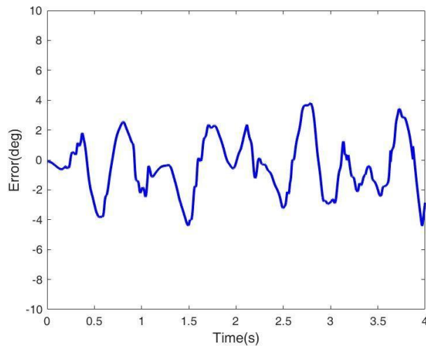
Figure 10. Trajectory tracking of the APK in man-machine hybrid model: (a) knee angular tracking; and (b) tracking error.
