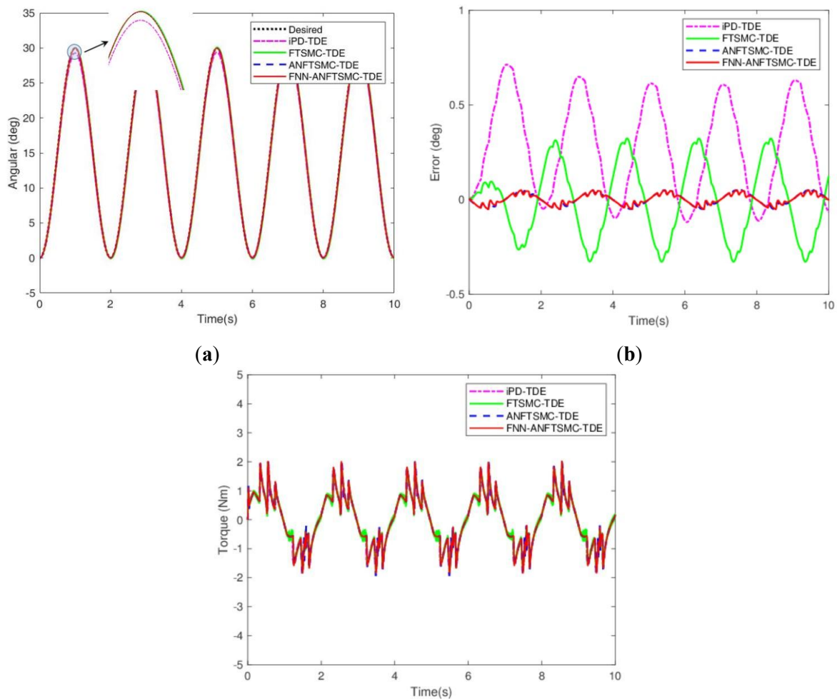
Figure 5. Simulation results of comparison among iPD-TDE, FTSMC-TDE, ANFTSMC-TDE, and FNN-ANFTSMC-TDE: (a) trajectory tracking; (b) trajectory error; and (c) control torque.
