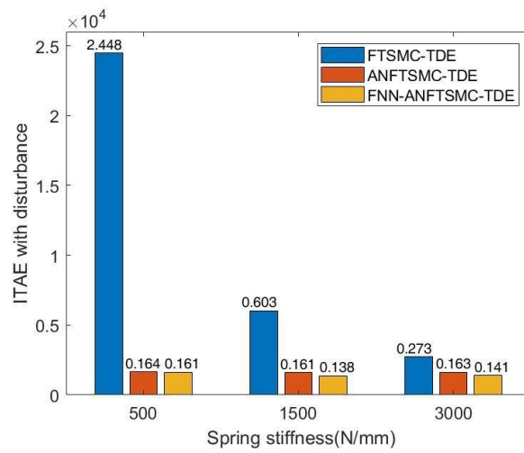
Figure 8. Simulation results of ITAE among FTSMC-TDE, ANFTSMC-TDE, and FNN-ANFTSMC-TDE under different joint stiffnesses: (a) ITAE without disturbance; and (b) ITAE when \tau_{d1} and \tau_{d2} occur.
