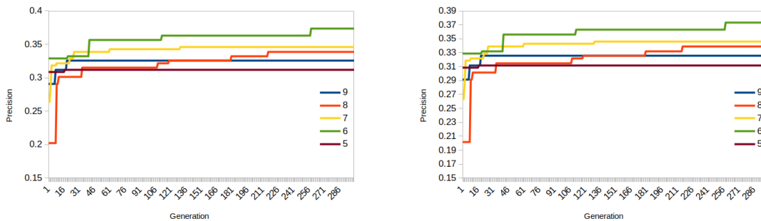
Figure 1. Precision of best individual over generations on Netscience data set. On the X axis the generation g , and on the Y axis the precision value of the best individual in the population at generation g . Each line shows the evolution dynamics on a specific fold.
