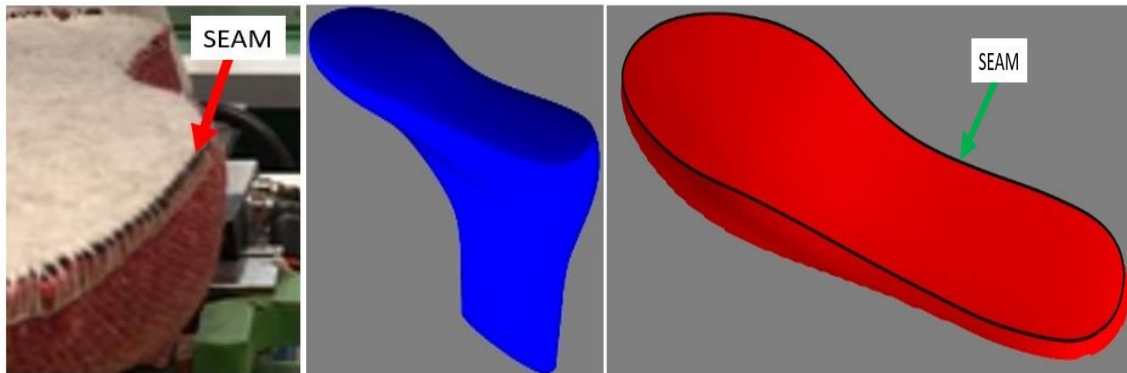
Figure 2. (a) Shoe upper. (b) STL file of shoe upper. (c) Reference glue deposition trace.
