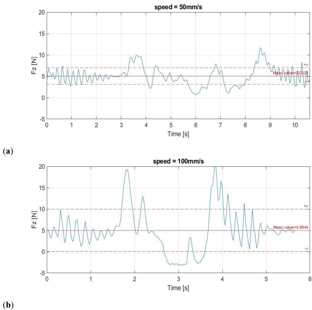
Figure 10. Contact force results for the cell layout with mobile shoe upper and fixed extruder. TM Robot. (a) Speed 50 mm/s. (b) Speed 100 mm/s.
