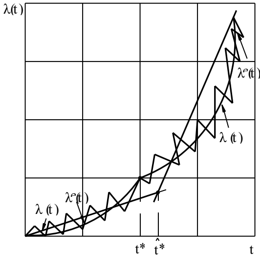
Fig. 1. The nature of the change in the frequency of failures occurring in electric submersible pumps: \lambda_1(t) , \lambda_2(t) – theoretical and \lambda_1^e(t) , \lambda_2^e(t) – empirical failure rates
